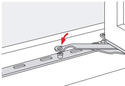
Figure 11: Bottom hinge oiling locations
