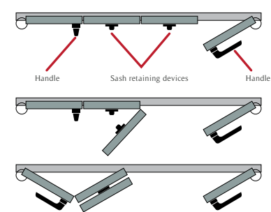
Figure 40: Opening of bifolding doors
