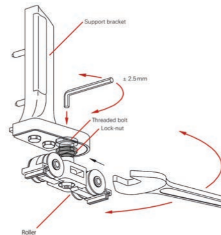
Figure 42: Adjusting the sash roller
