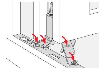
Figure 10: Bottom hinge oiling locations
