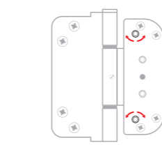
Figure 29: Horizontal adjustment
