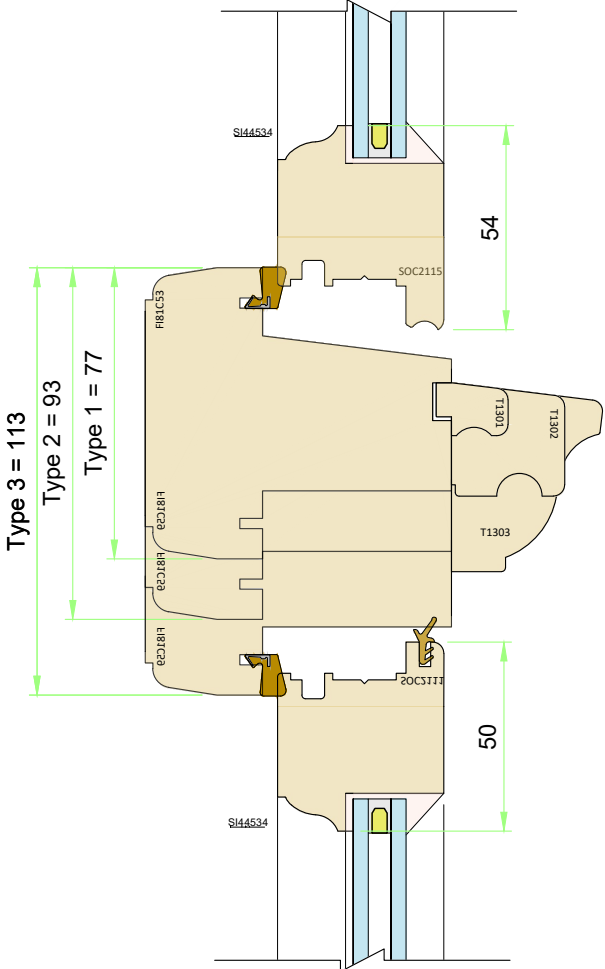
Transom drip options Scale 1:2
