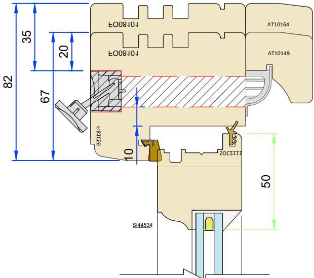
Frame vent (standard design) Scale 1:2
