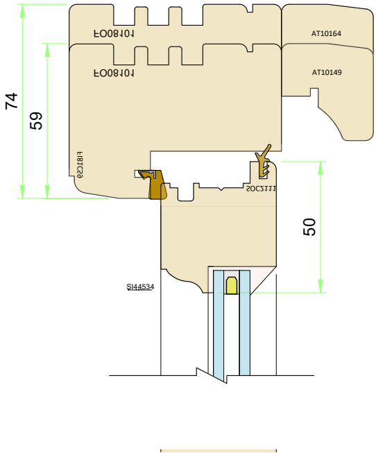
Head drip options Scale 1:2
