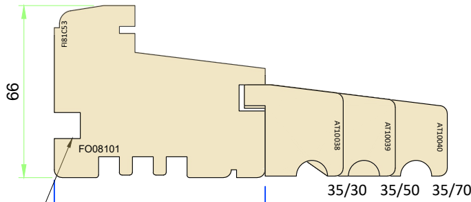
Cill Extension Options - 35mm Scale 1:2
