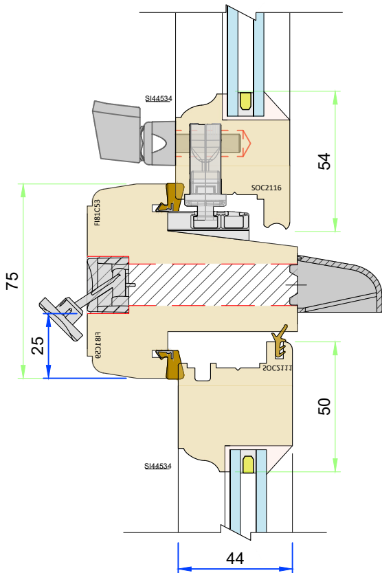
Section C-C - Transom - Showing trickle vent Scale 1:2
