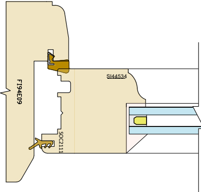
Bevel Extended Profile
