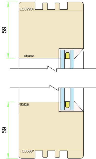
Section J-J - Direct Glazed Options Scale 1:2
