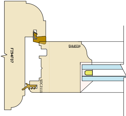
Extended Frame Options - PExt Ovolo profile
