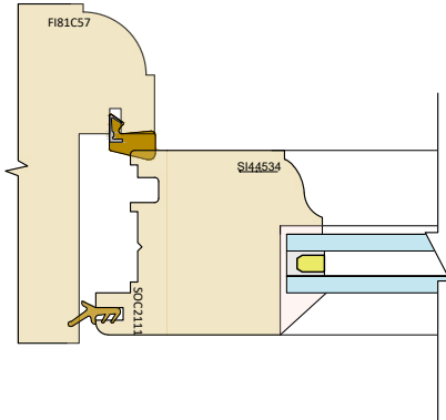
Extended Frame Options - BExt Ovolo profile
