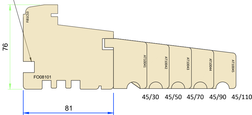
Cill Extension Options - 45mm
