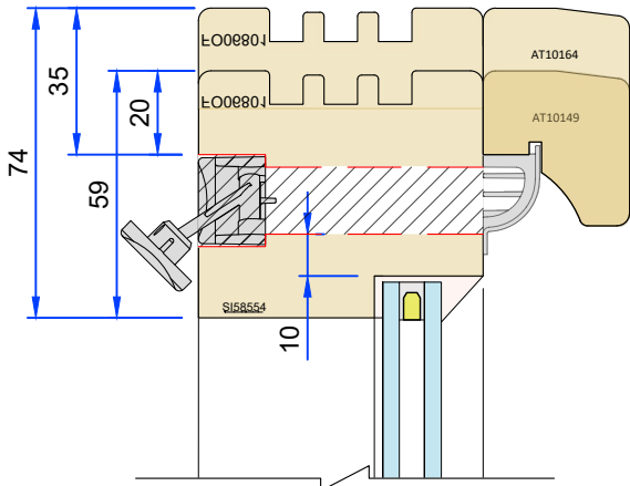
Direct glazed vent option
