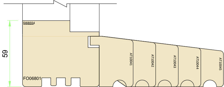
Cill Extension Options - 45mm
