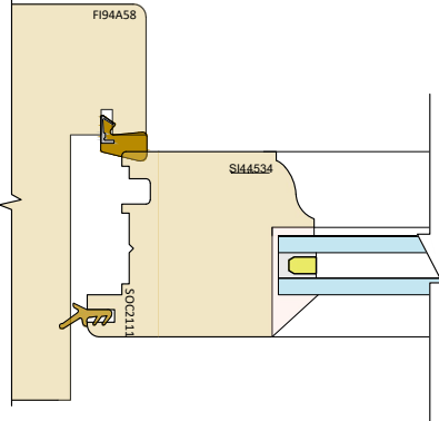
Pencil round profile
