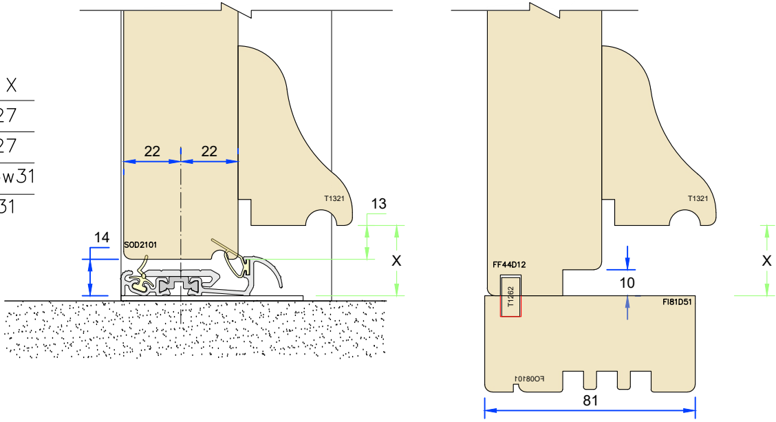
Standard low threshold option
