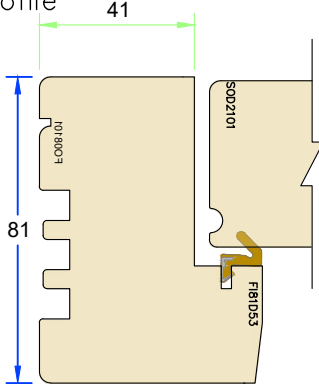
81mm frame – Standard profile
