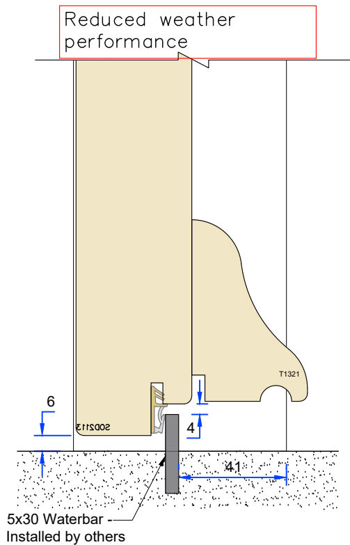
Waterbar threshold option
