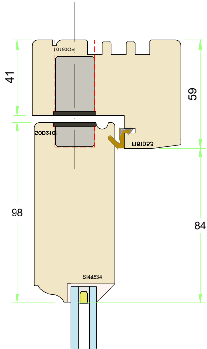
Typical head location
