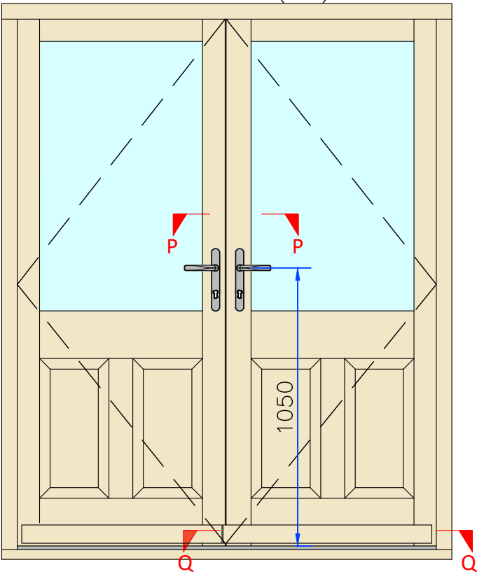
French Doors – Outside View (1: 20)
