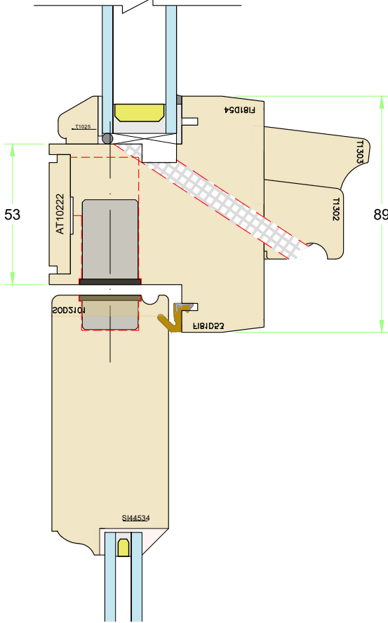
Typical transom location
