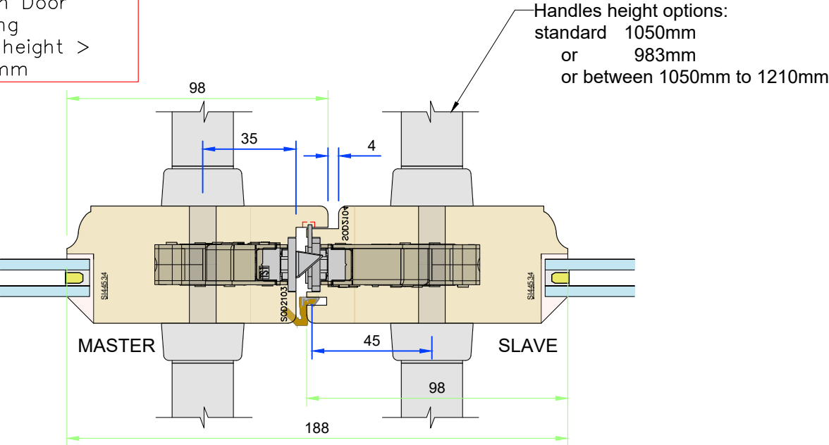
French door locking options
