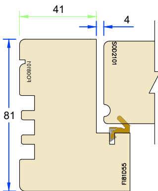
81mm frame – Square profile
