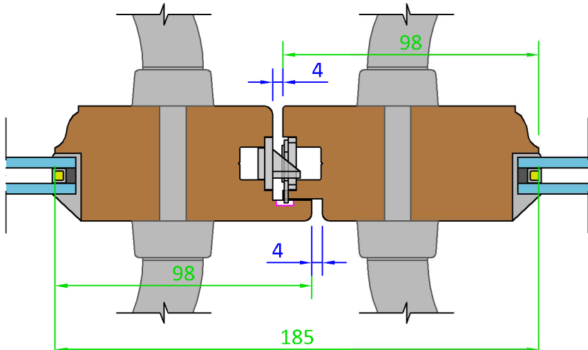
Section K-K French Door Meeting ThumbBolt Option - (Scale 1:2)
