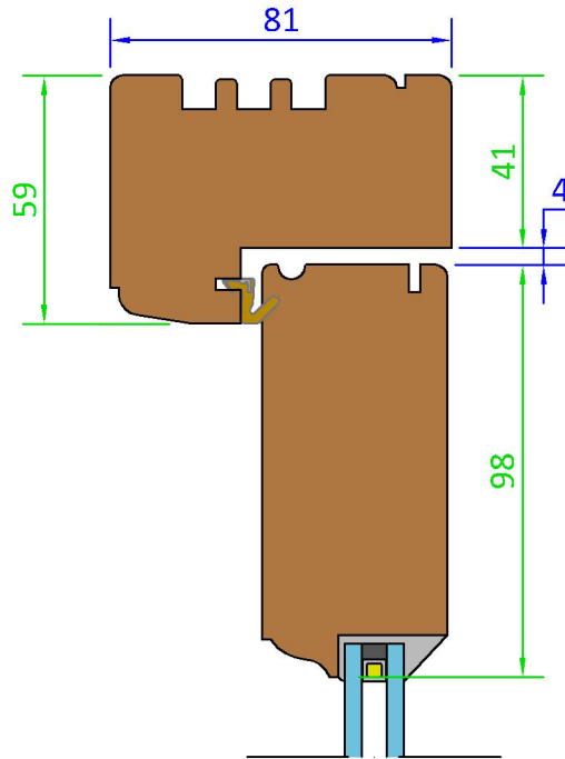
Section C-C - Head Detail (Scale 1:2)
