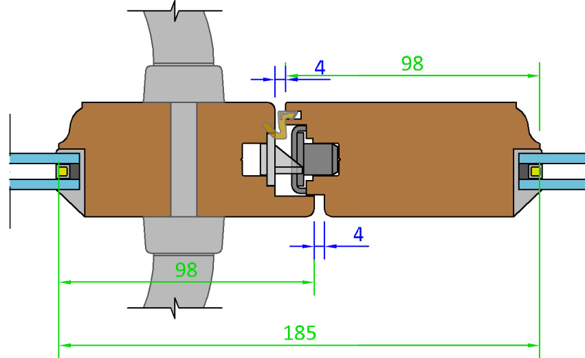
Section K-K French Door Meeting - (Scale 1:2)
