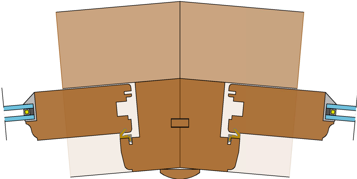
156-179° Segmented Bay
