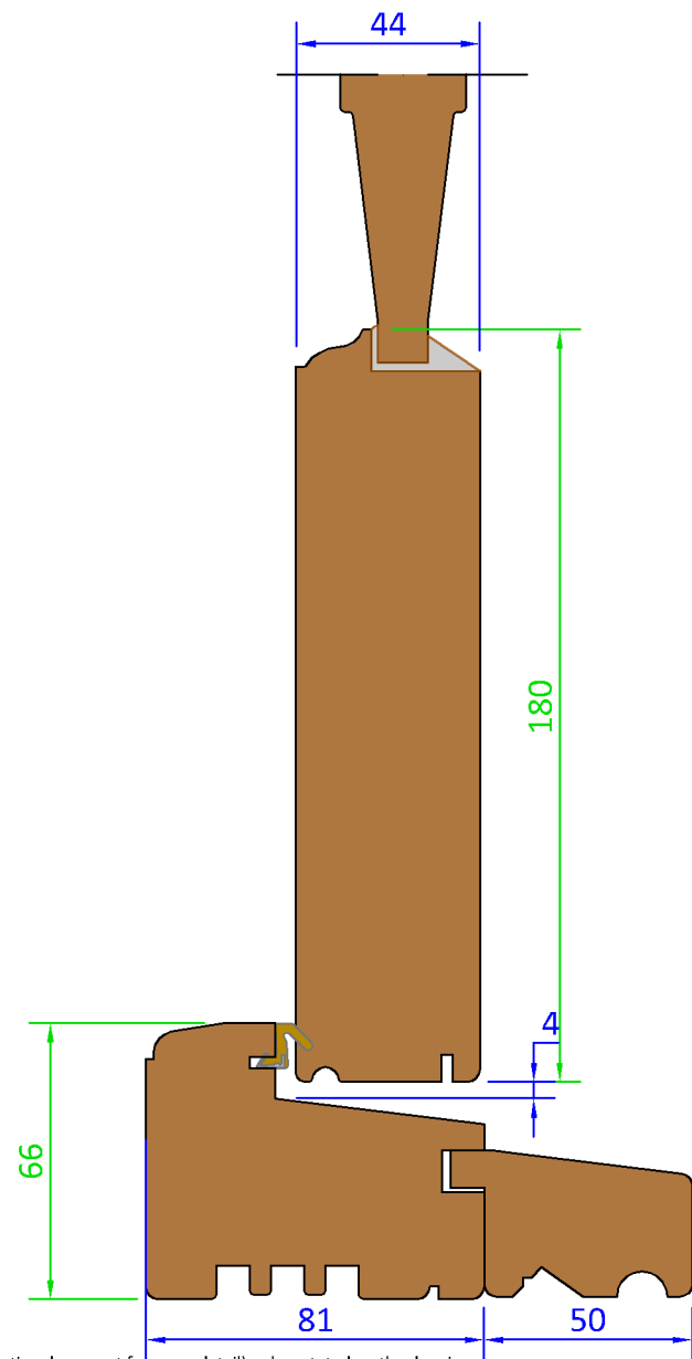
Section D-D - Cill Detail (Scale 1:2)
