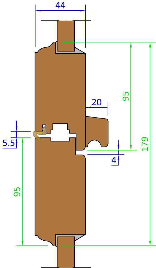
Stable Door Meeting J-J (Scale 1:2)
