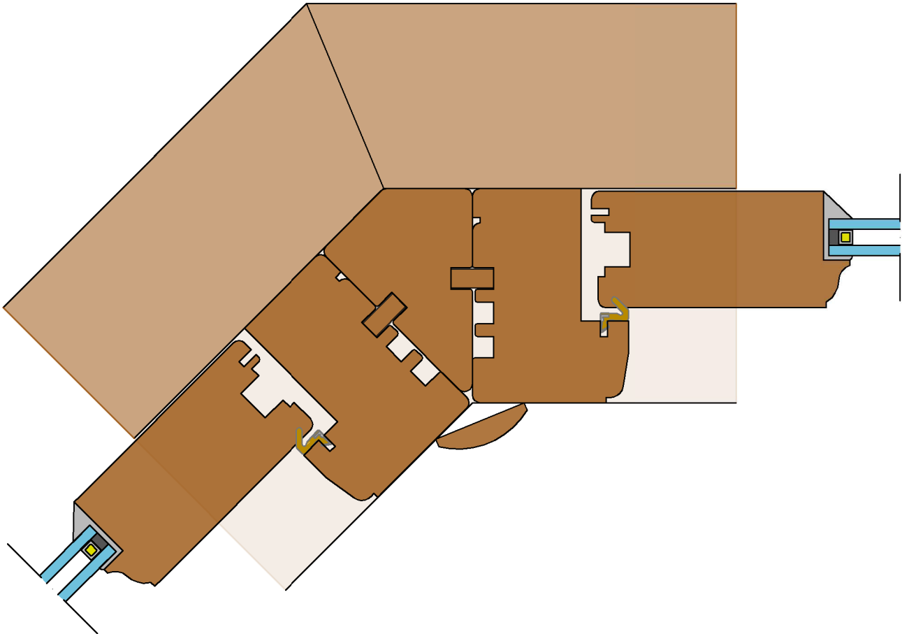
91-155° Angled Corner Post
