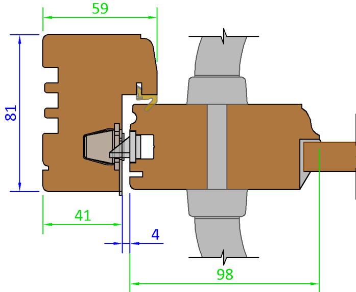
Stable Door Handle L-L (Scale 1:2)
