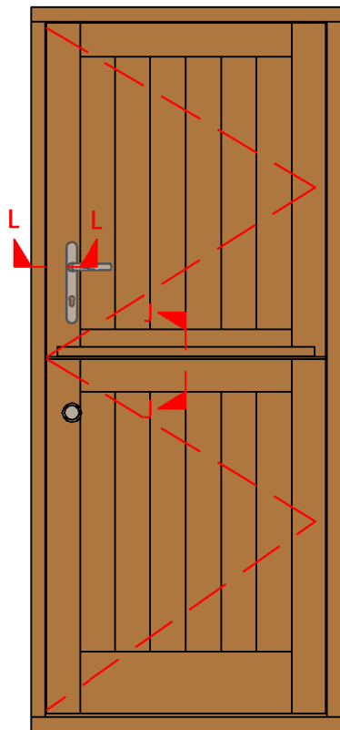
Stable Door - Outside View (Scale 1:40)
