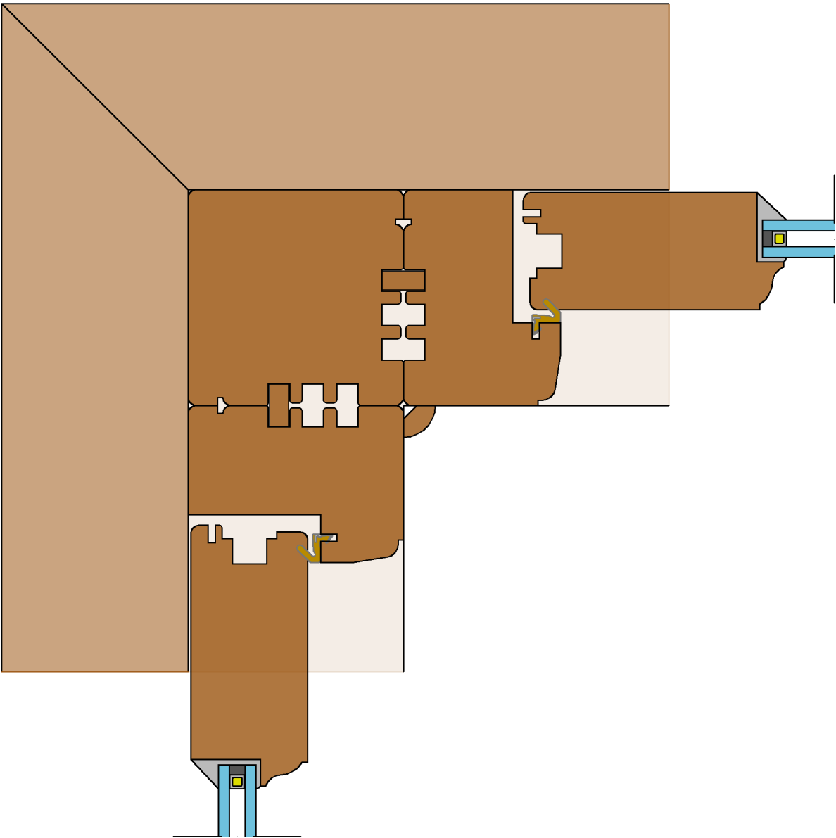
90° Corner Post
