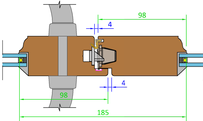
Section K-K French Door Meeting - (Scale 1:2)
