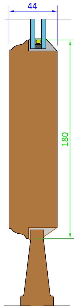
Section E-E - Mid Rail Detail (Scale 1:2)
