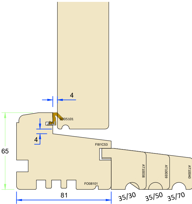
For 35mm extension
