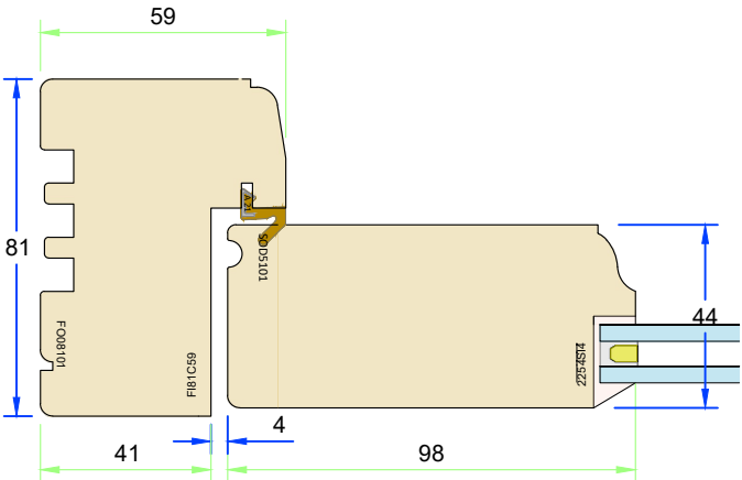
94mm frame - Ovolo profile
