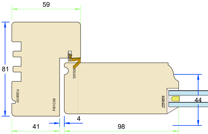
94mm frame - Pencil round profile
