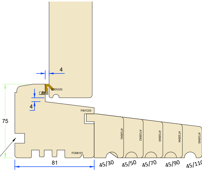
For 45mm extension
