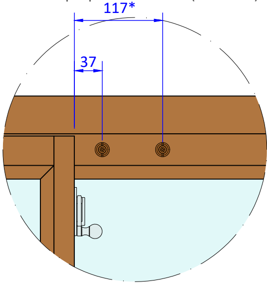
Sash Stop Option 'A' & 'K' - (Scale 1:5)
