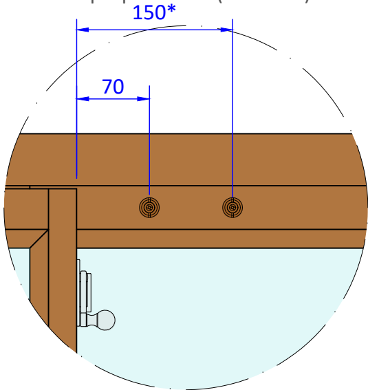
Sash Stop Option 'G' - (Scale 1:5)
