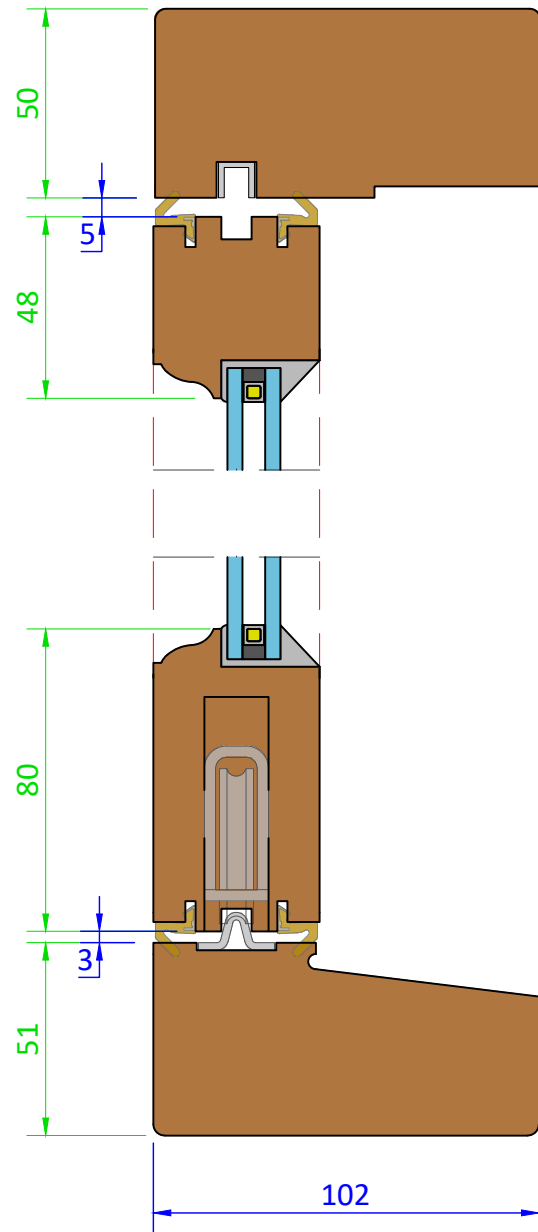
Section B-B - Cill Detail (Scale 1:2)
