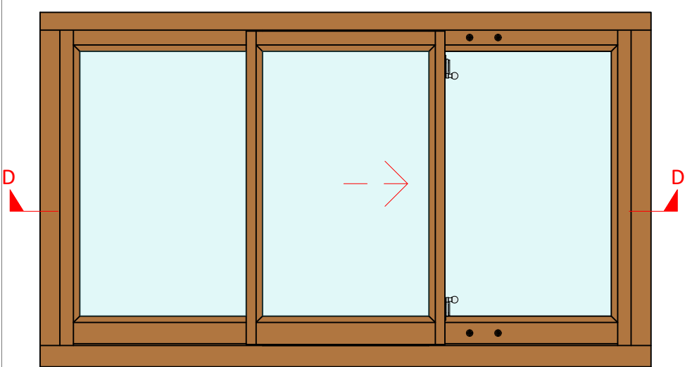
Inside View (Scale 1:15)
