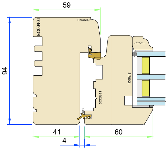
Section A-A - Jamb and mullion detail
