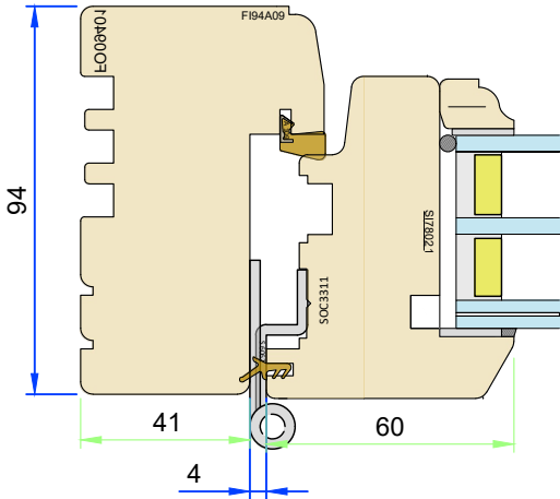
Butt Hinge option
