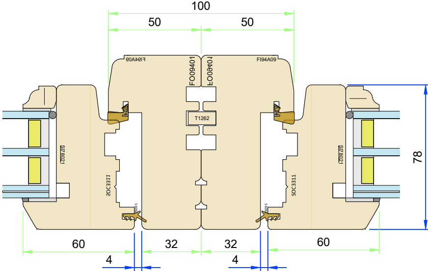
Section M-M - Jamb Connection Scale 1:2
