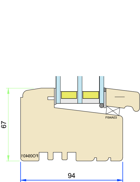
Section J-J - Direct Glazed Options Scale 1:2
