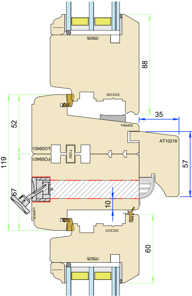
Horizontal frame connection incorporating trickle vents Scale 1:2
