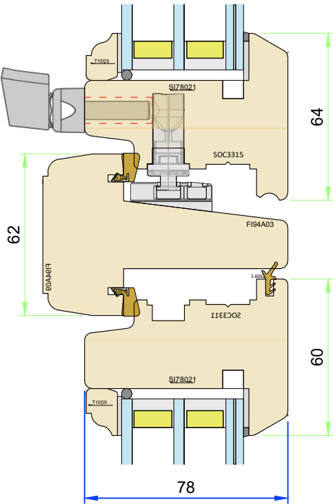
Section C-C - Transom detail
