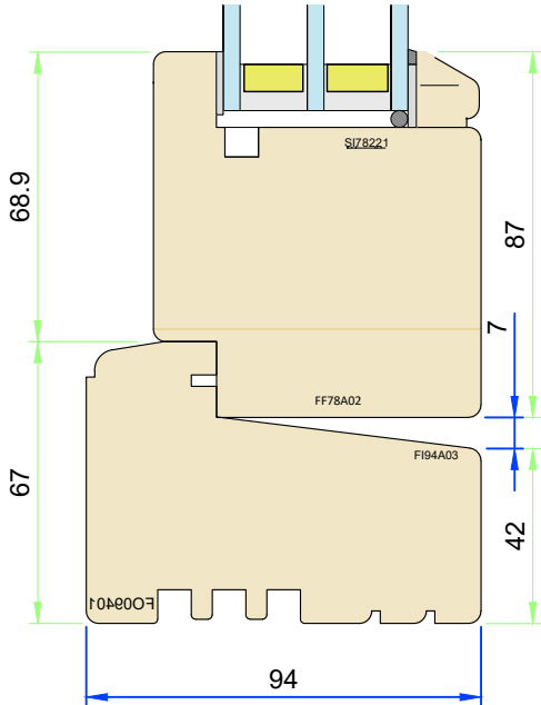
Section K-K - Direct glazed head options Scale 1:2
