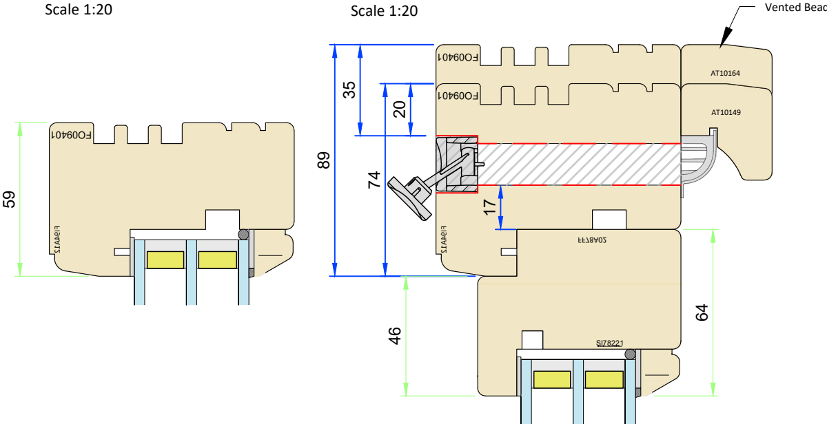
Direct Glazed Elevation Scale 1:20
