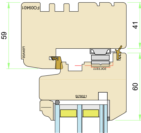
Section G-G - 16mm Hinge Option
