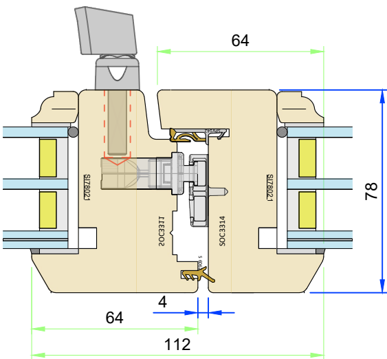
Section D-D - French Window
