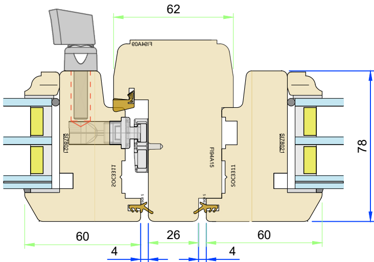
Section E-E - False Mullion
