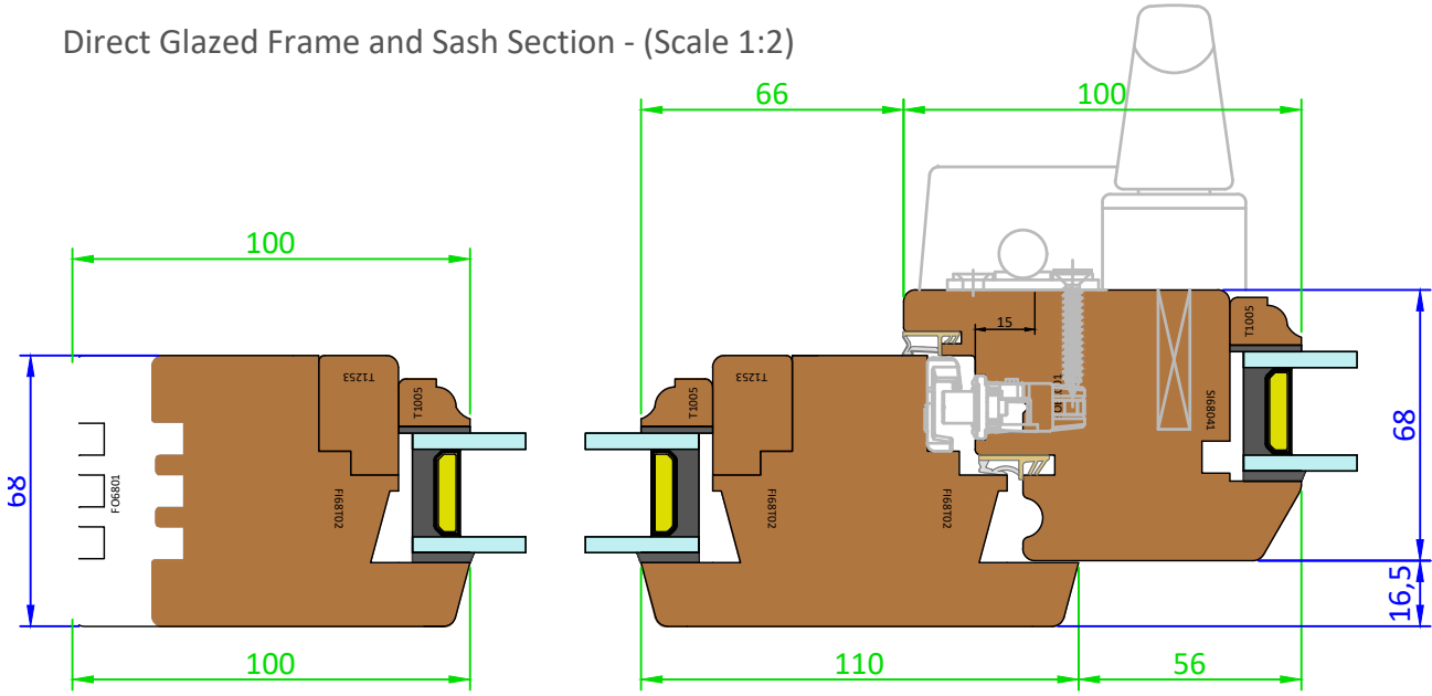
Meeting Rail Section - (Scale 1:2)
