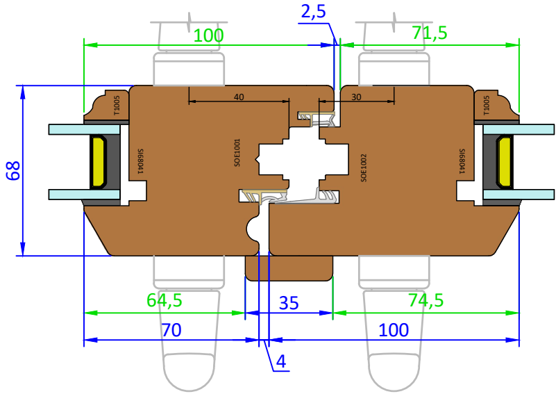
Fixed Mullion Section - (Scale 1:2)
