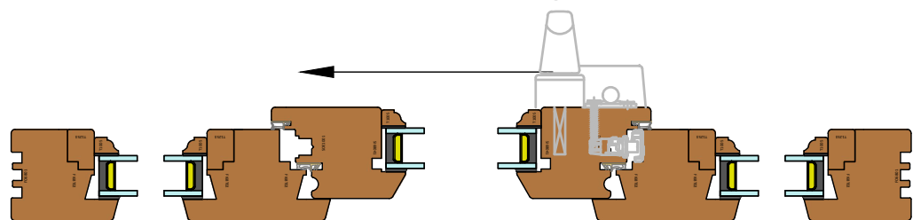
Scheme G - Slide Left with Double Fixed Glazing Panels (DS12-??)
