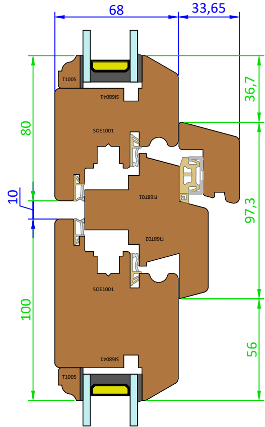
Timber Transom Option - (Scale 1:2)
