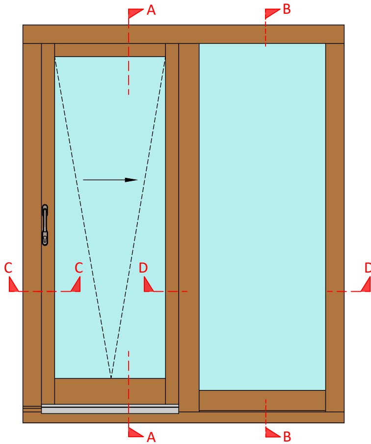
Elevation 2 - Inside View
