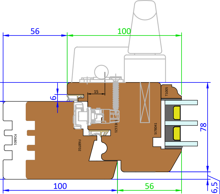
68mm Frame and 78mm Sash - Standard Profile
