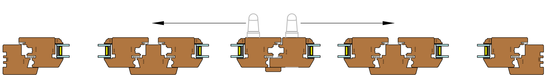
Scheme C - Double Sliding with Fixed Mullion and Double Turn-Only Sashes (DS12-CF)
