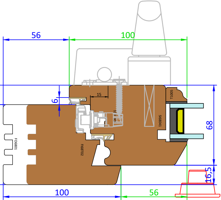
68mm Frame and 78mm Sash - Standard Profile
