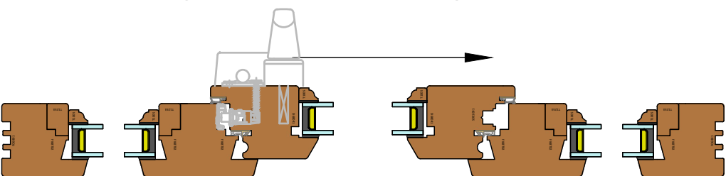
Scheme G - Slide Right with Double Fixed Glazing Panels (DS12-??)
