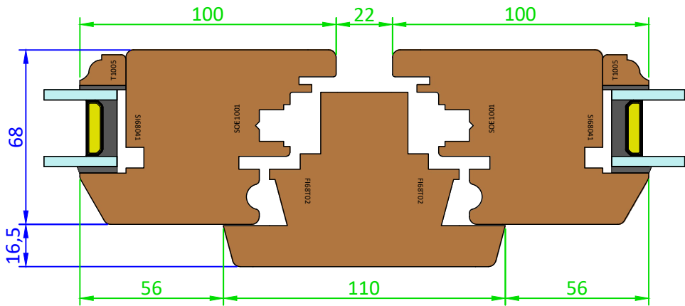
Fixed Mullion Section - (Scale 1:2)
