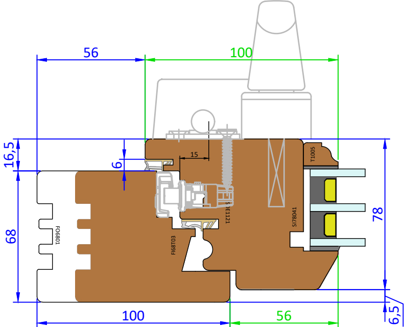
68mm Frame and 78mm Sash - Pencil Round Profile
