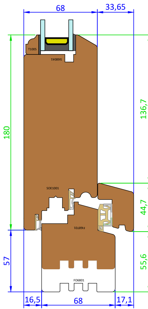
Timber Cill Option - (Scale 1:2)
