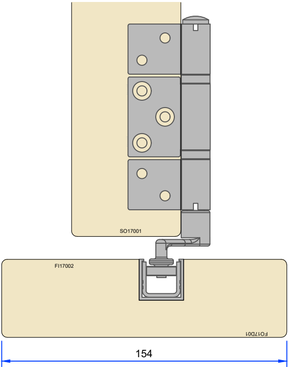
Timber cill option - internal use only
