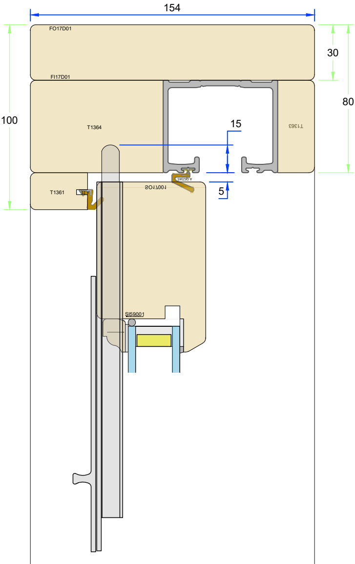
Head detail showing deadbolt
