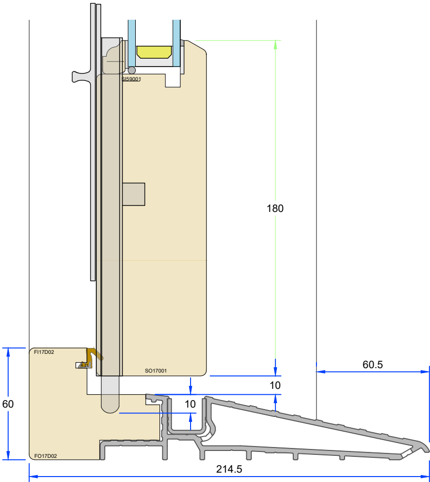
Cill detail showing deadbolt
