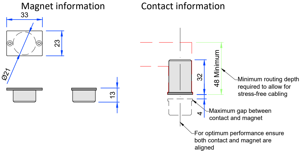
Flush quick fit door contact details
