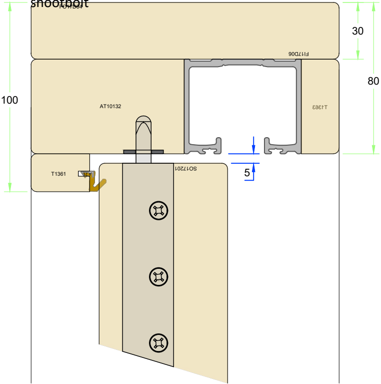
Head detail showing position of the top twinlock shootbolt
