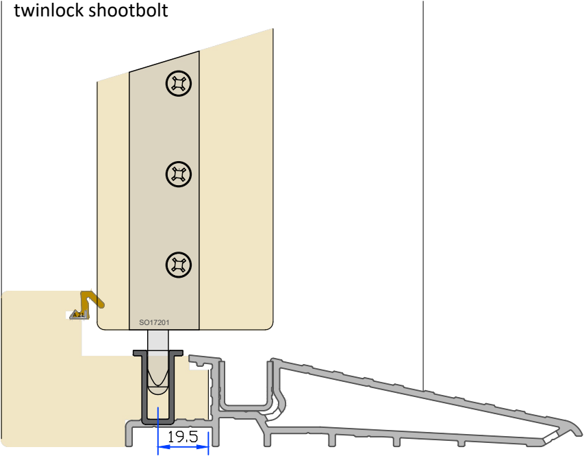
Cill detail showing the position of of the bottom twinlock shootbolt
