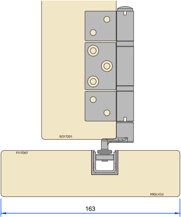
Timber cill option - internal use only
