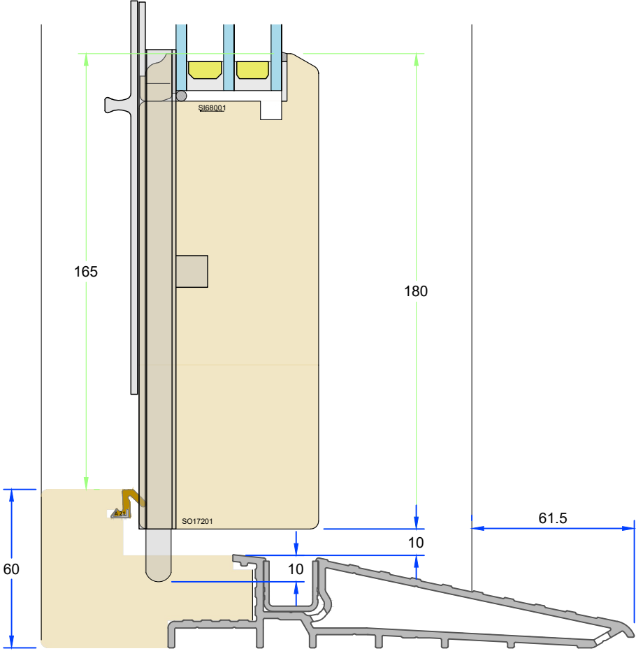
Cill detail showing keyed dropbolt
