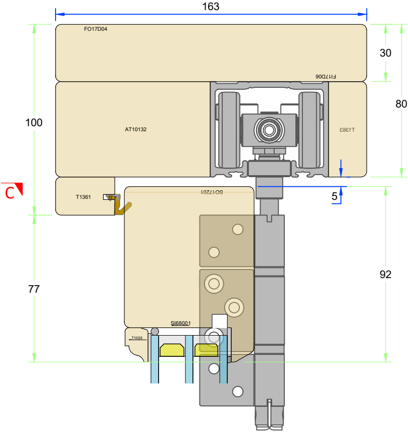
Section A-A - Head detail
