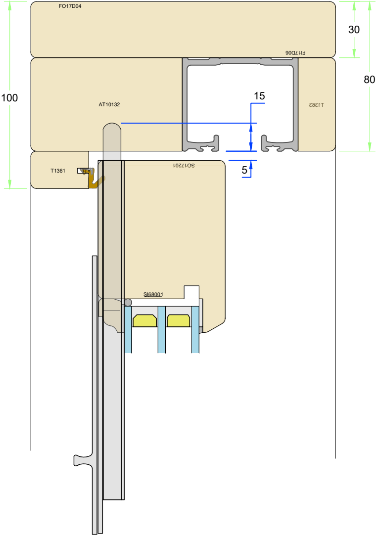
Head detail showing position of the top twinlock shootbolt
