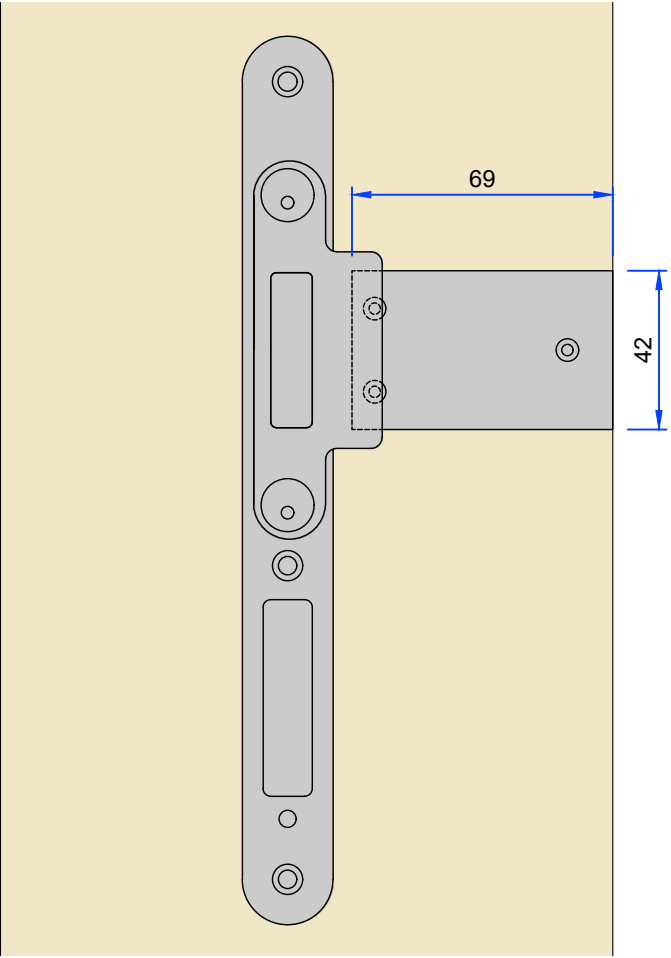
Timber cill option - internal use only
