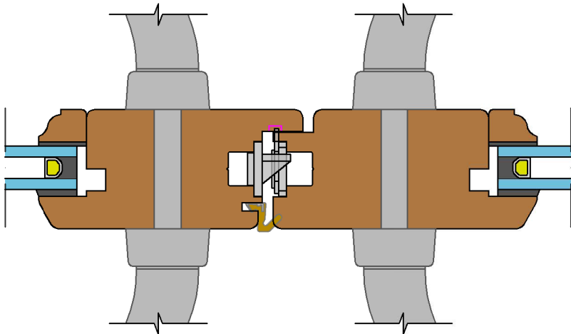
Thumb Bolt Lock Option - (Scale 1:2)
