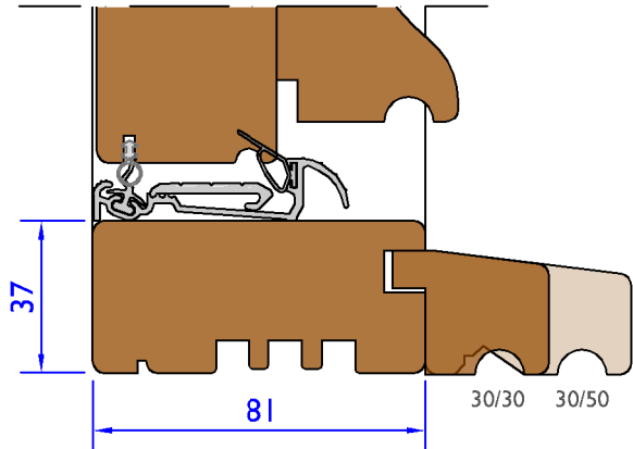
Cill Extension For 35 mm Extension
