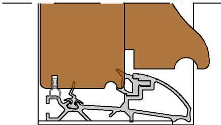
Low Threshold Cill Option 3 - (Scale 1:2)
