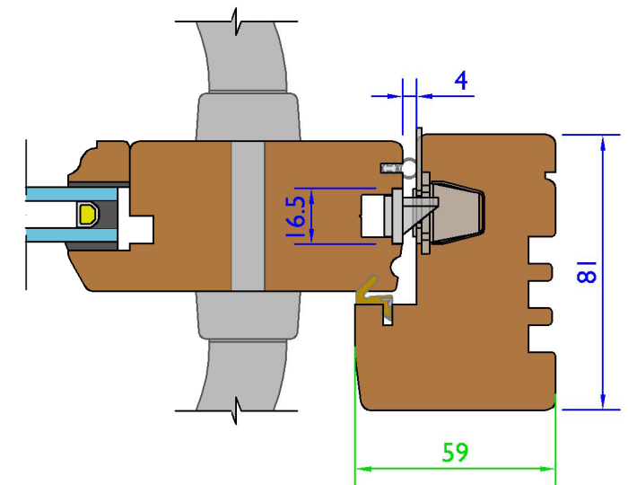
Section M-M Stable Door Lock and Frame - (Scale 1:2)
