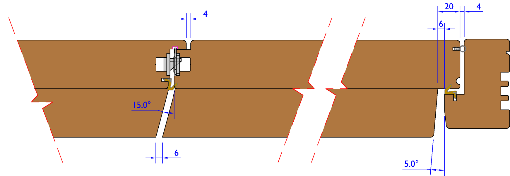
Section L-L - Timber Weather Bar Fitting - (Scale 1:2)
