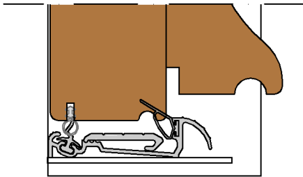
Low Threshold Cill Option 1 - (Scale 1:2)
