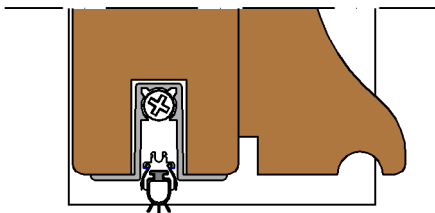
Low Threshold Cill Option 2 - (Scale 1:2)
