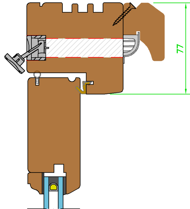
Frame Vent Option (Slide In/Grille Out) - (Scale 1:2)
