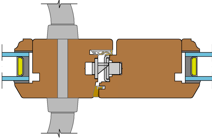
French Door Meeting Concealed Lock Option - (Scale 1:2)
