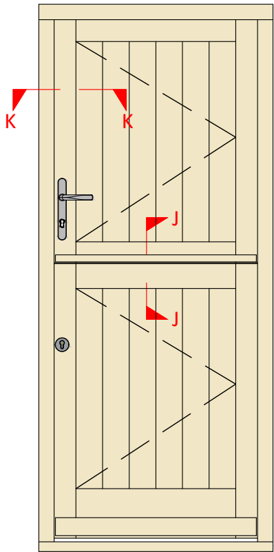
Stable Door – Outside View
