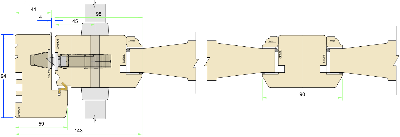
Section E-E – Jamb and vertical rail
