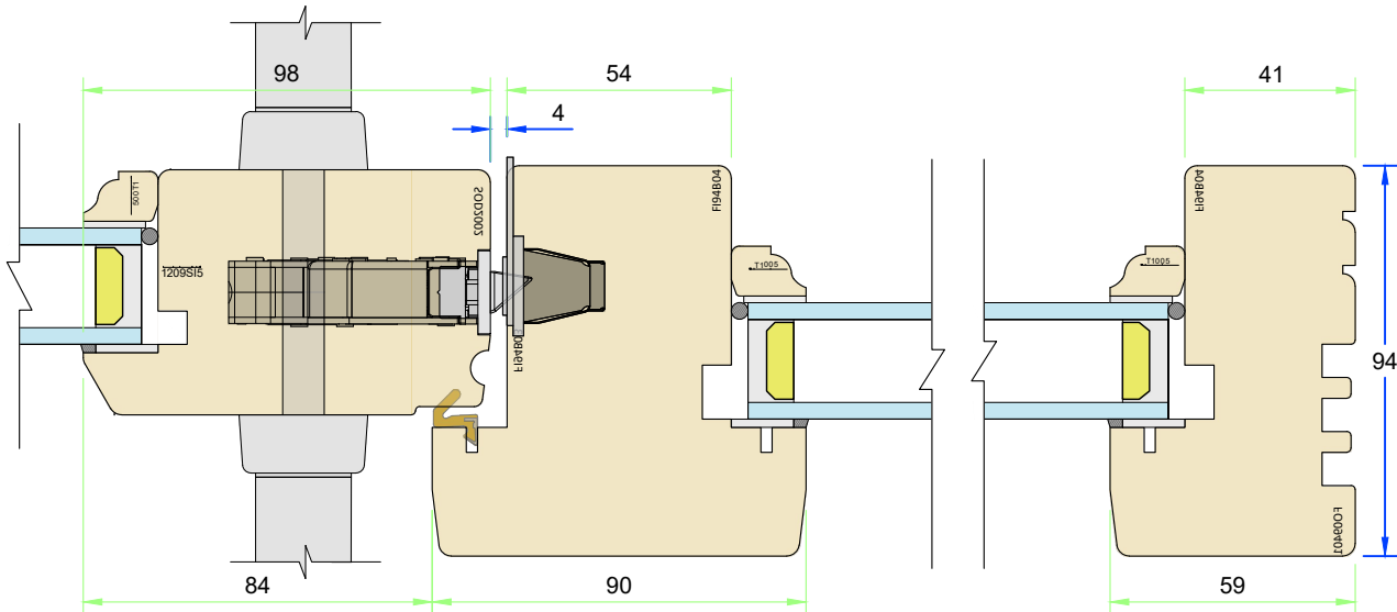
Section H–H
