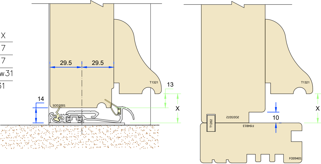
Standard low threshold option
