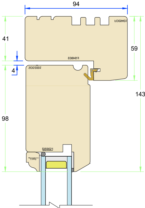
Section A-A – Head detail
