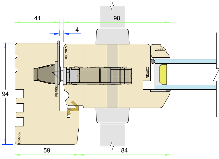
Section K–K – Stable door lock and frame
