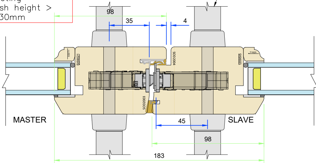
French door locking options
