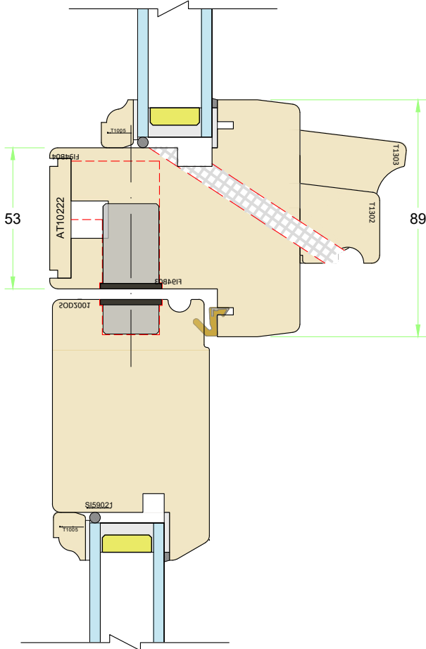
Typical transom location
