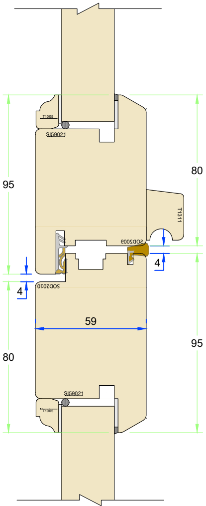
Section J–J – Stable door meeting
