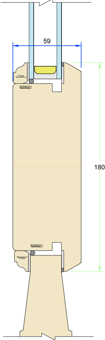
Section C-C – Midrail
