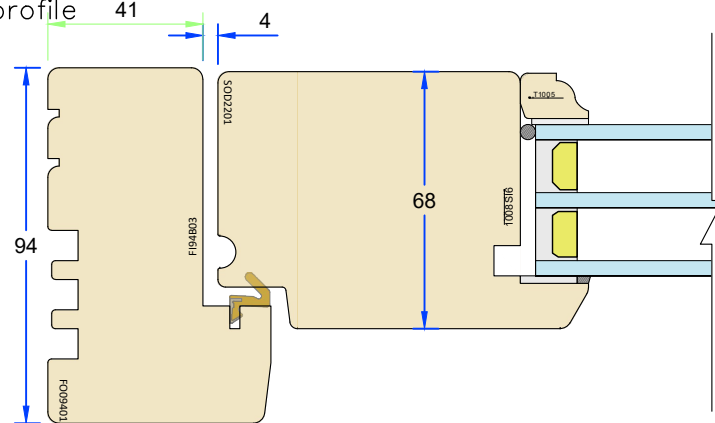
94mm frame – Pencil round profile
