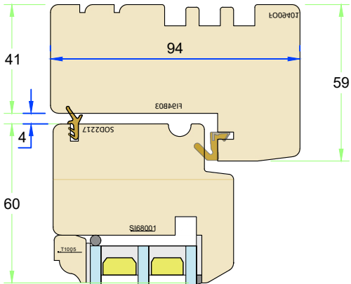
Section L-L
