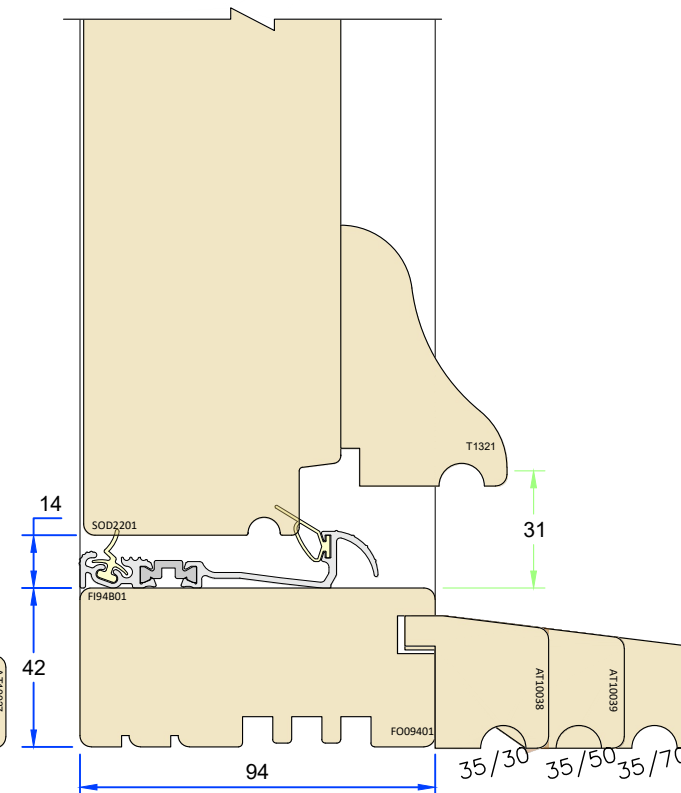
For 35mm extension
