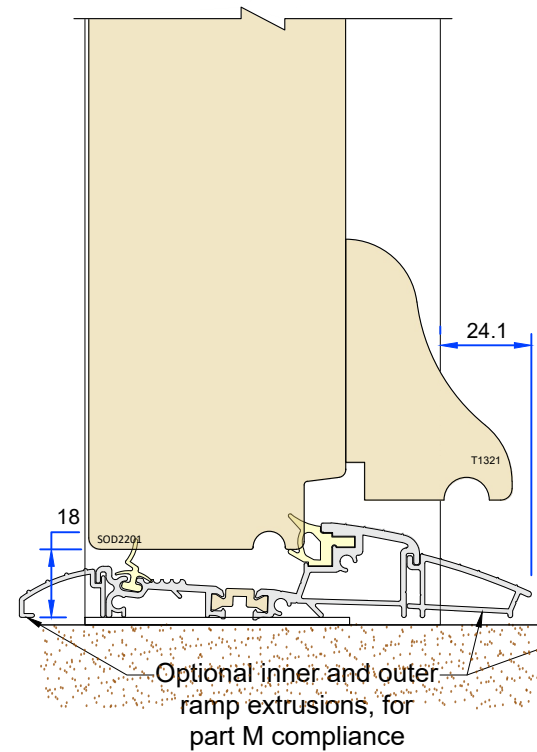
For 35mm extension
