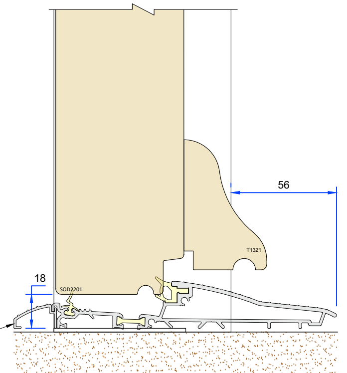
Aluminum low threshold option
