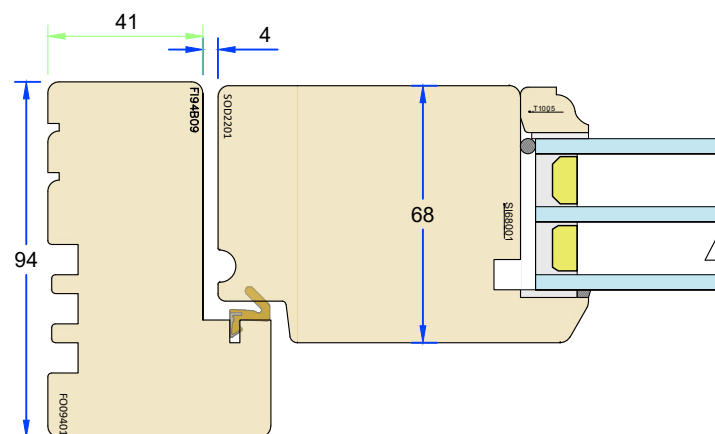
94mm frame – Pencil round profile
