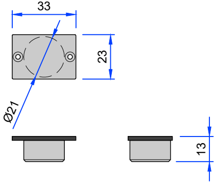
Flush quick fit door contact details
