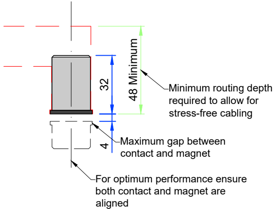
Flush quick fit door contact details
