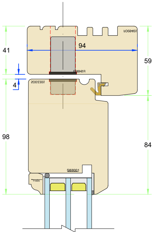
Typical head location
