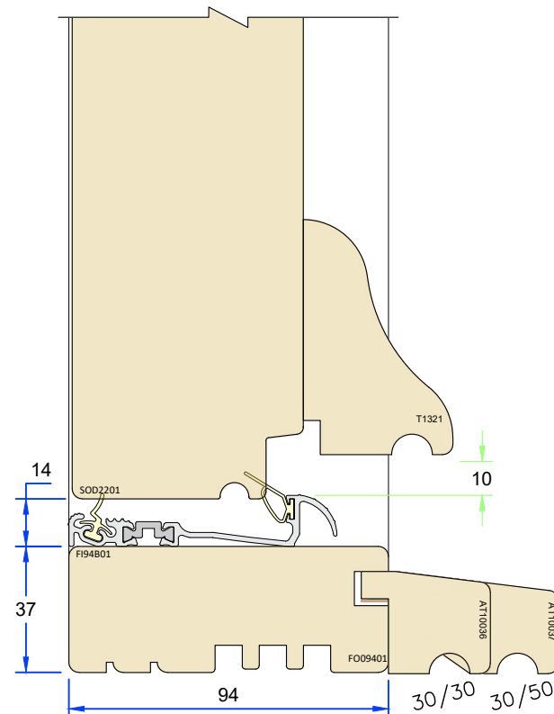
For 30mm extension
