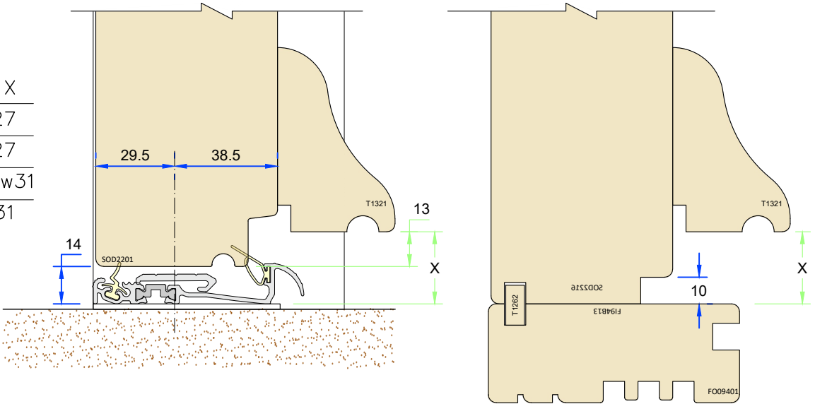
Standard low threshold option
