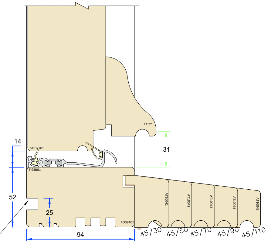
For 45mm extension
