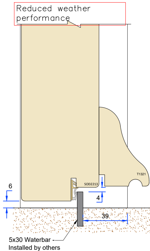
Waterbar threshold option
