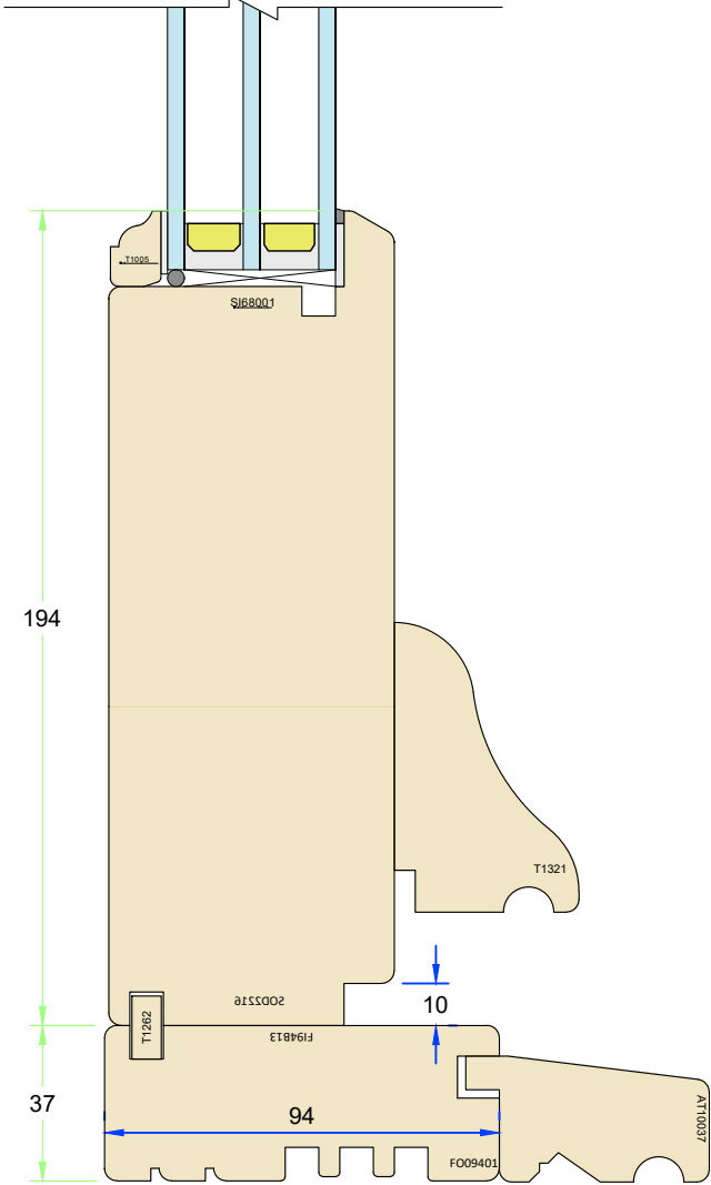
Section M-M
