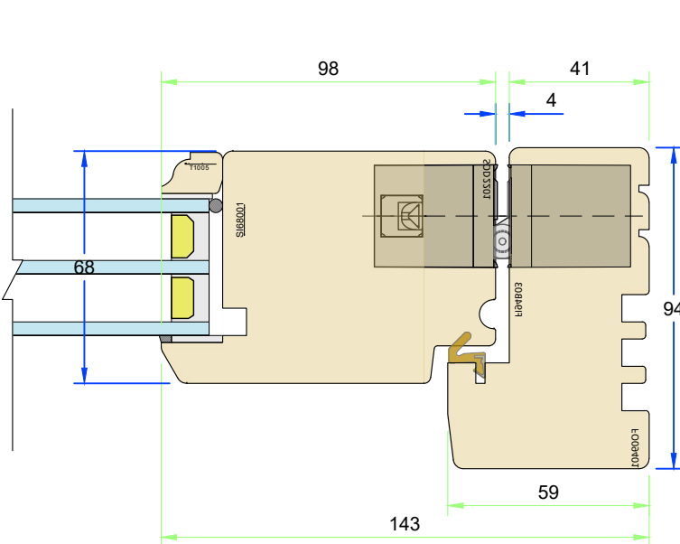
Section D-D – Concealed hinge option
