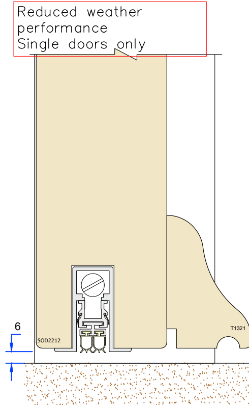
Dropdown seal threshold option
