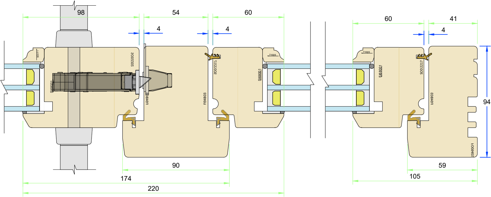
Section N-N
