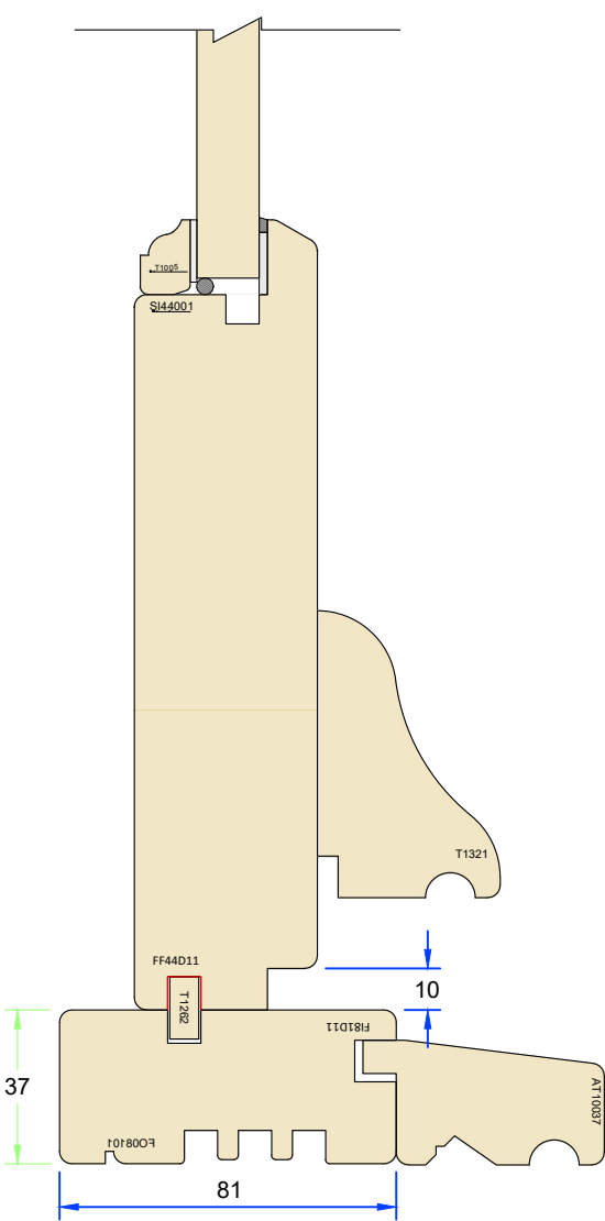
Section G-G
