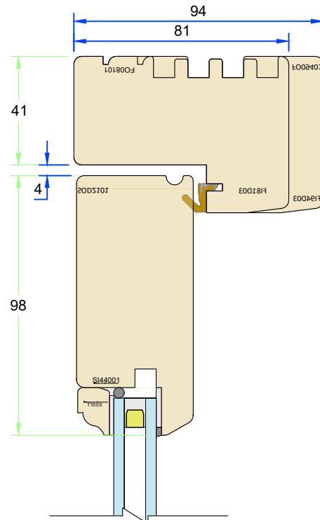
Section A-A - Head detail
