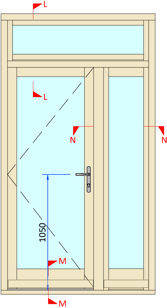
Fixed sash fanlight & sidelight - Outside View
