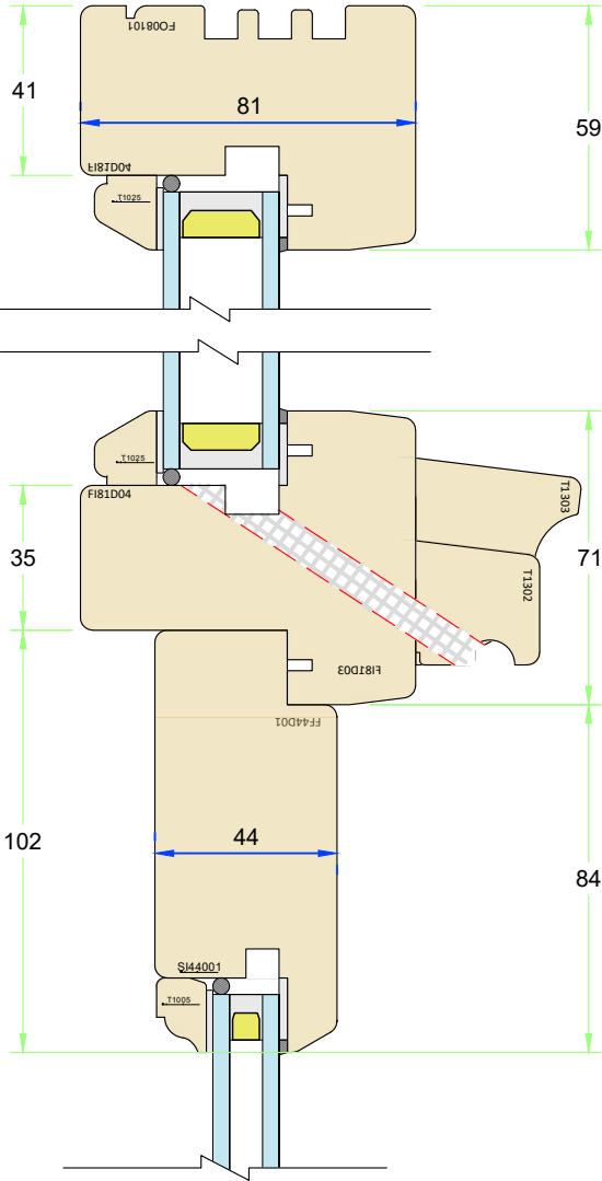
Section F-F
