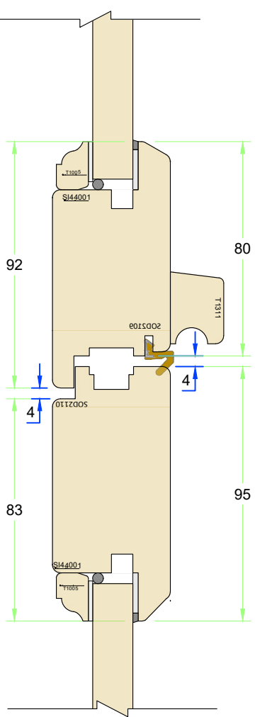
Section J-J - Stable door meeting
