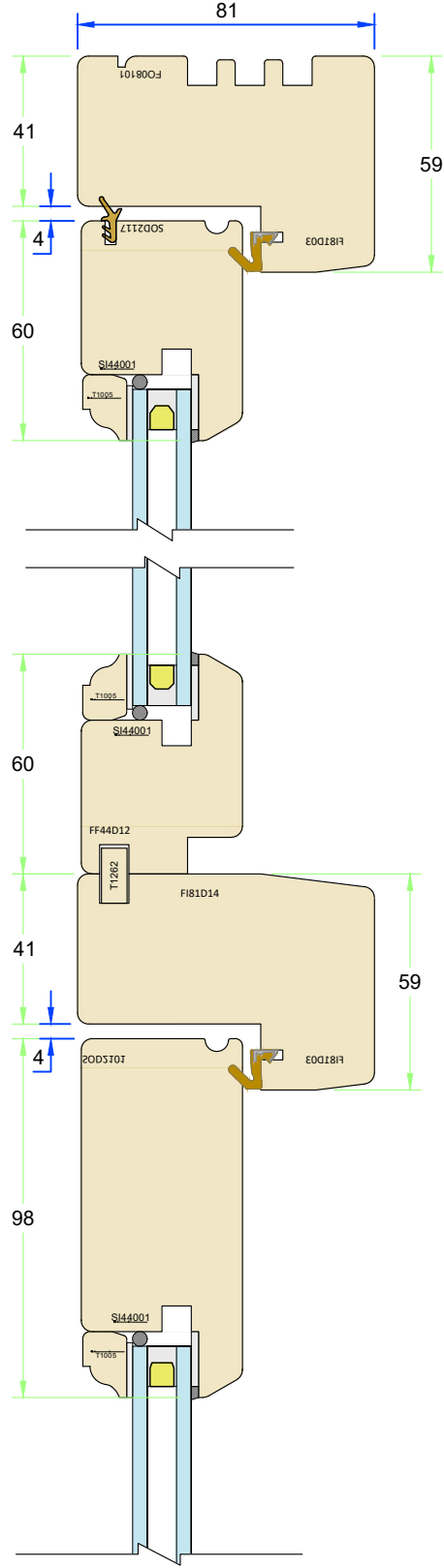
Section L-L
