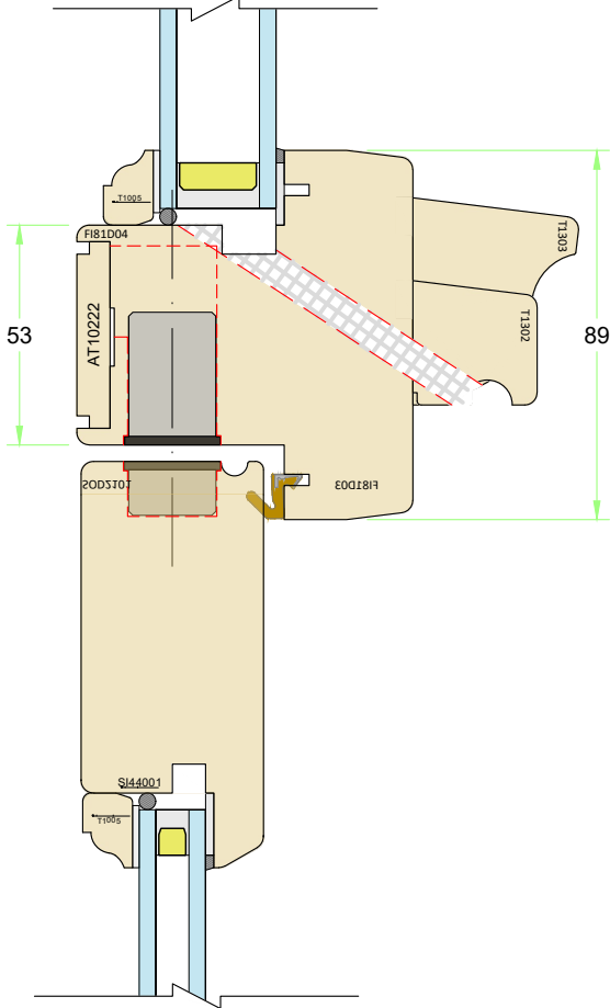
Typical transom location
