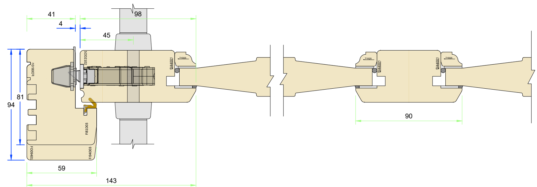
Section E-E - Jamb and vertical rail
