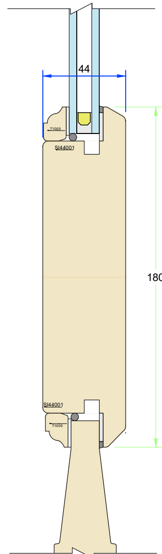
Section C-C - Midrail
