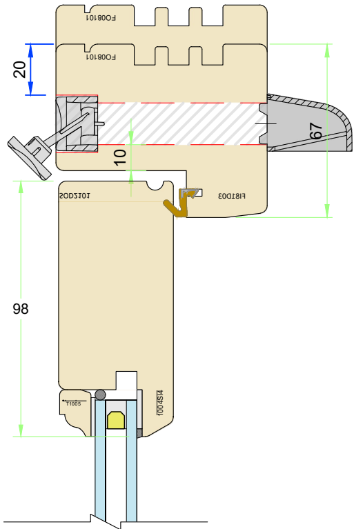
Frame vent - with optional canopy
