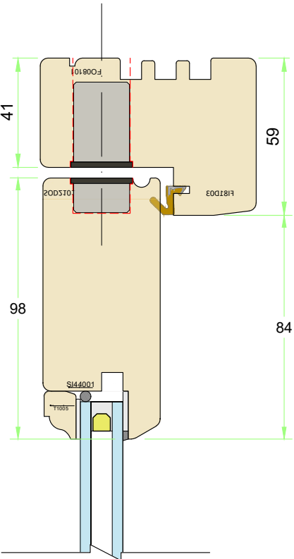
Typical head location
