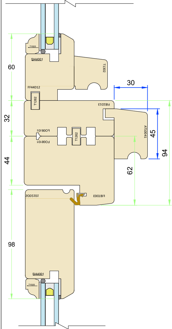
Filler rail options
