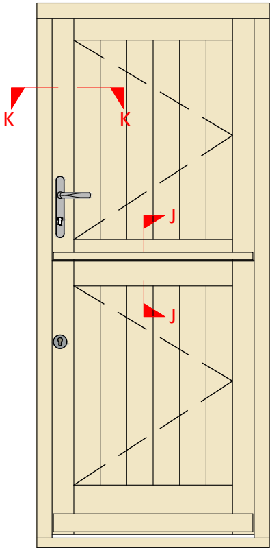
Stable Door - Outside View
