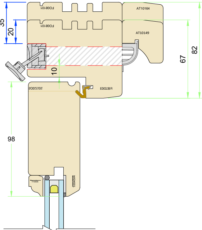
Frame vent - standard design
