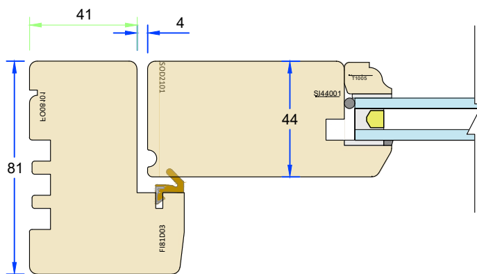
81mm frame - Standard profile
