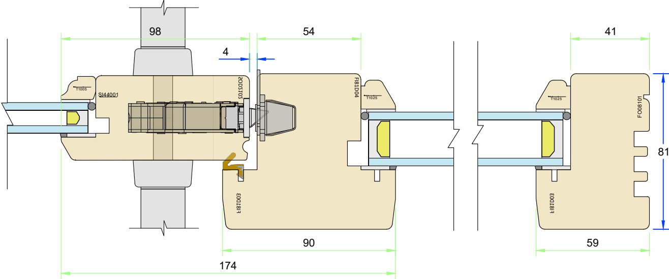
Section H-H
