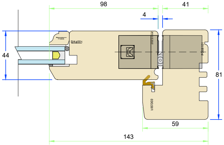
Section D-D - Concealed hinge option
