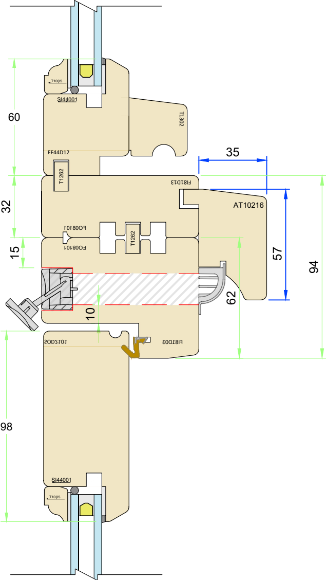
Horizontal frame connection incorporating trickle vents
