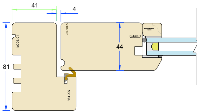
81mm frame - Pencil round profile
