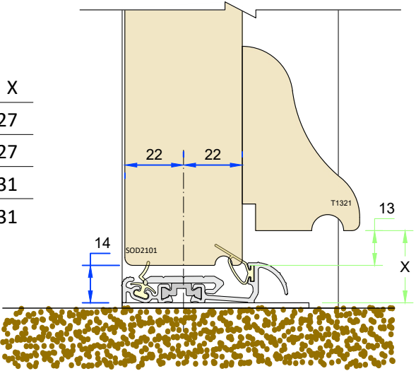
Standard low threshold option
