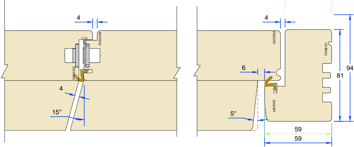
French Meeting Timber Weather Bar
