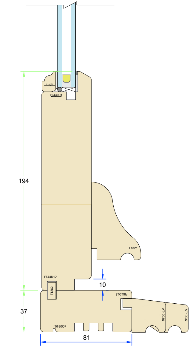
Section M-M
