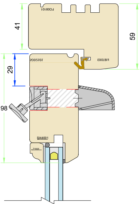
Sash vent - with canopy
