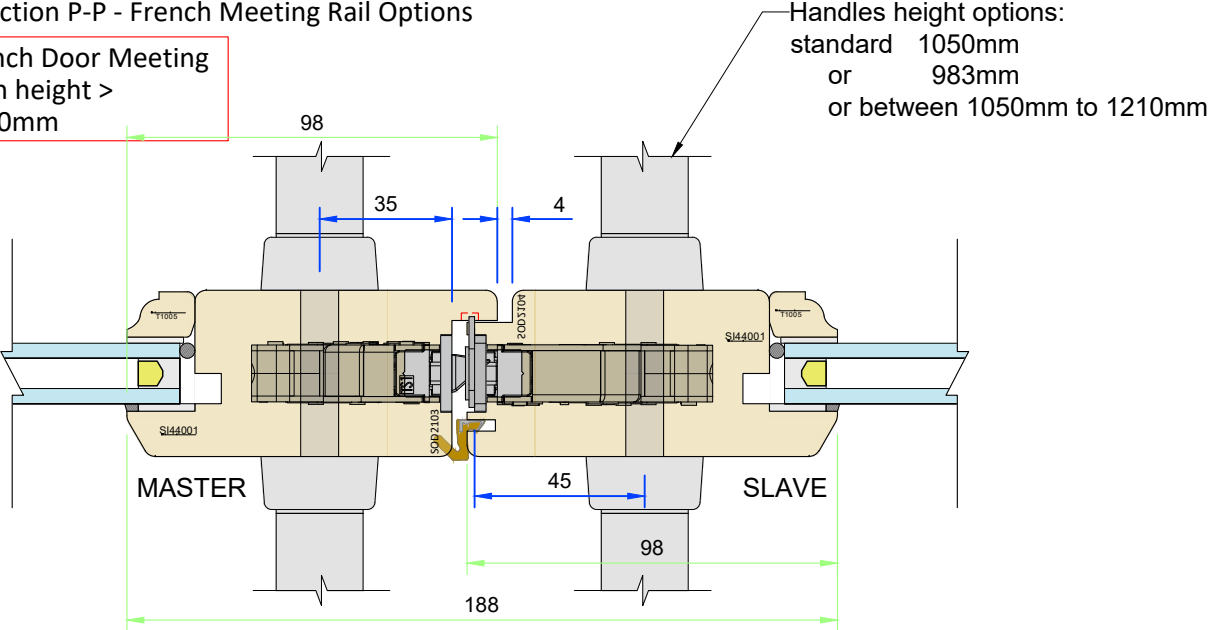
French door locking options
