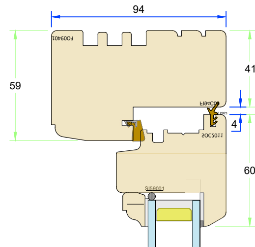
Section L-L - Typical head/jamb detail
