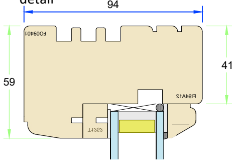
Section G-G - Typical head/jamb detail
