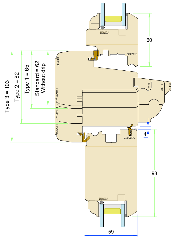
Transom drip detail
