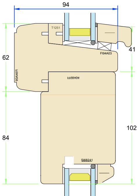
Section H-H - Head filler rail detail
