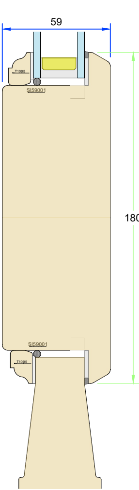
Section C-C - Midrail
