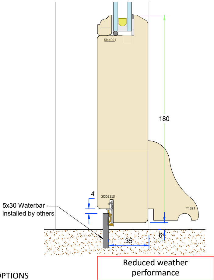
94mm frame - Pencil round profile
