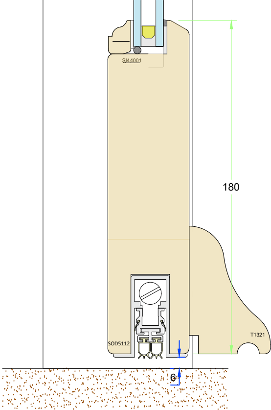
Dropdown seal threshold option
