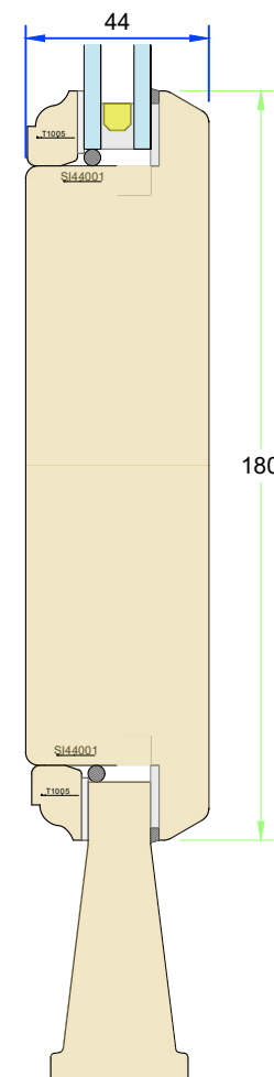
Section C-C - Midrail
