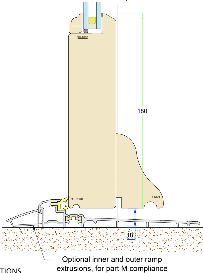
Aluminum low threshold option
