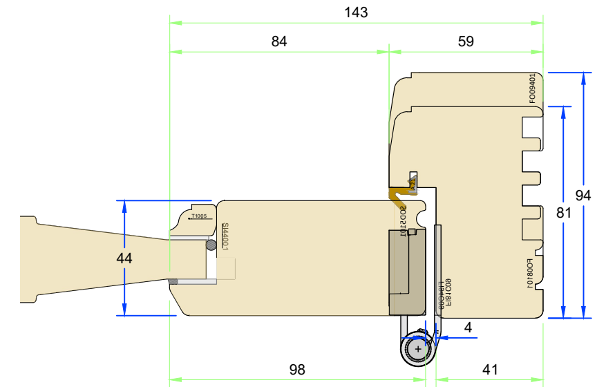
Section D-D - Hinge detail
