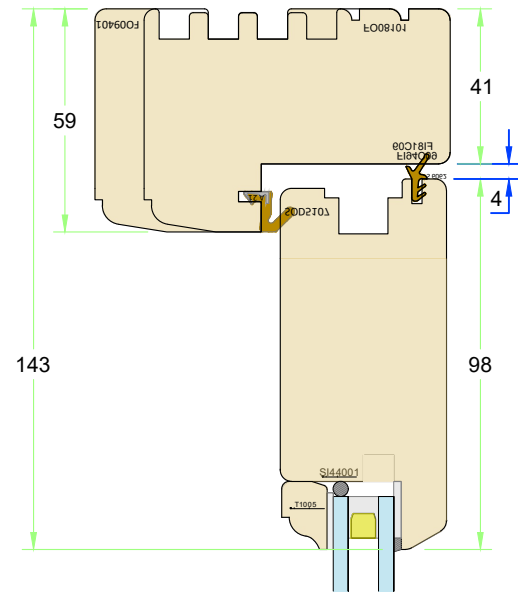
Section A-A - Head detail
