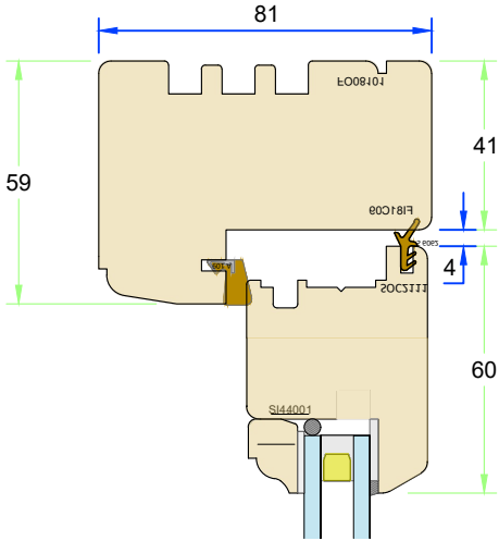
Section L-L - Typical head/jamb detail
