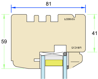
Section G-G - Typical head/jamb detail
