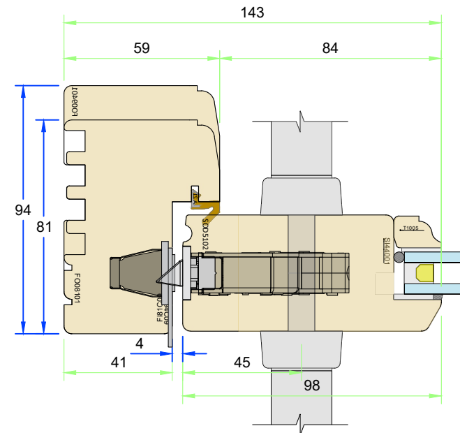
Section E-E - Jamb and lock
