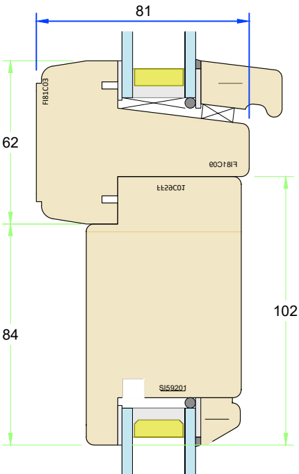
Section H-H - Head filler rail detail
