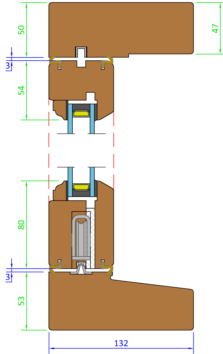
Section B-B - (Scale 1:2)
