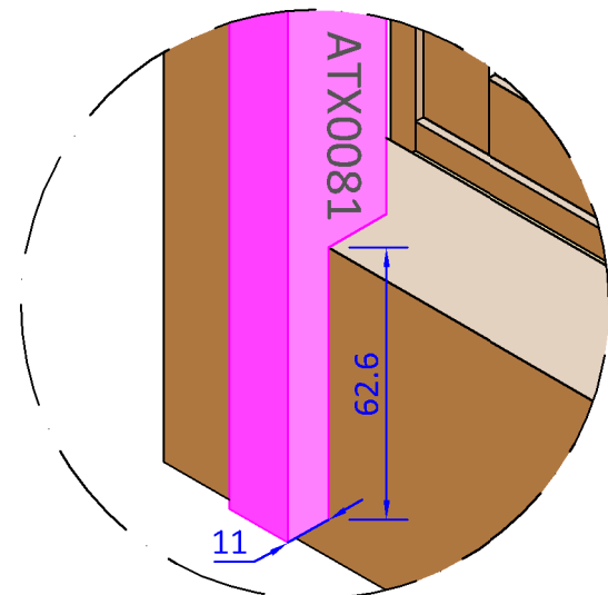
Fixed Sash Meeting Rail Strip detail - (Scale 1:2)
