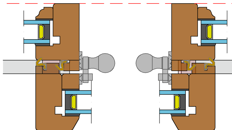
Section E-E - (Scale 1:2)
