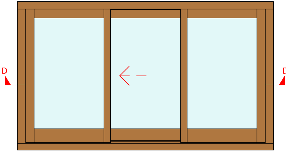
Scheme 'G' Outside View (Scale 1:15)
