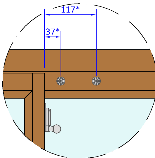
Sash Stop Option 'A' & 'K' - (Scale 1:5)
