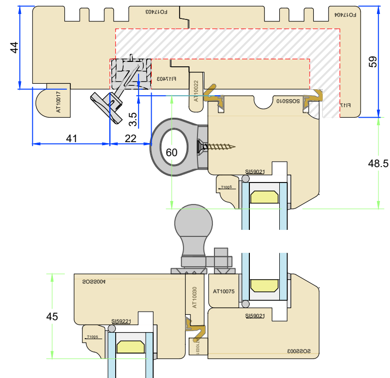
Section A-A - Head, Cill and Meeting Rails
