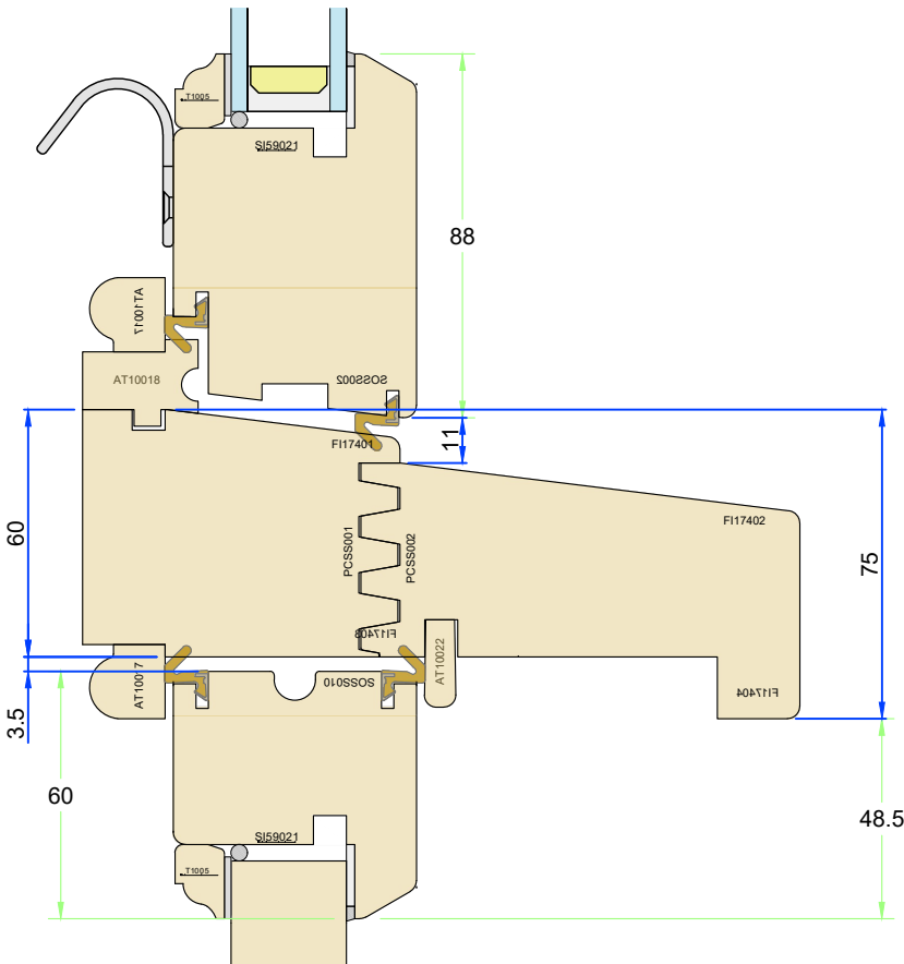
Section E-E - Low level transom detail
