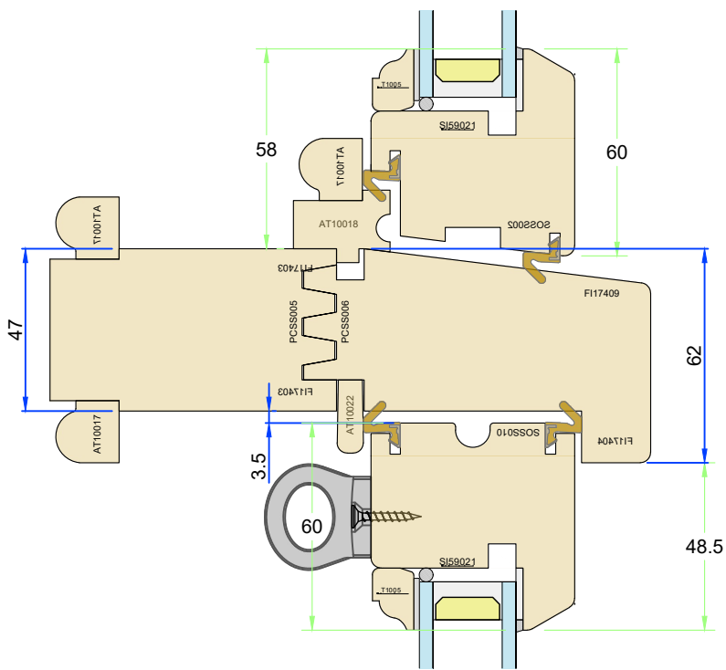
Section E-E - Low level transom detail
